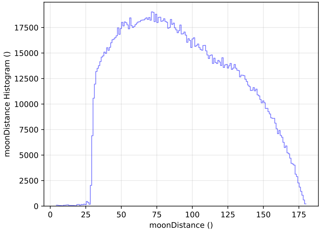
ddf_acor_sf15_lsf20_lsr20_v3.4_10yrs All sky all bands: moonDistance Histogram
