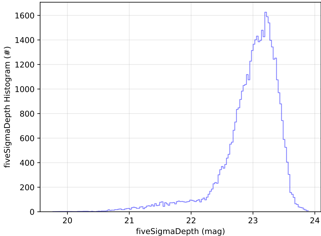
ddf_acor_sf15_lsf20_lsr20_v3.4_10yrs Yr 1 z band: fiveSigmaDepth Histogram
