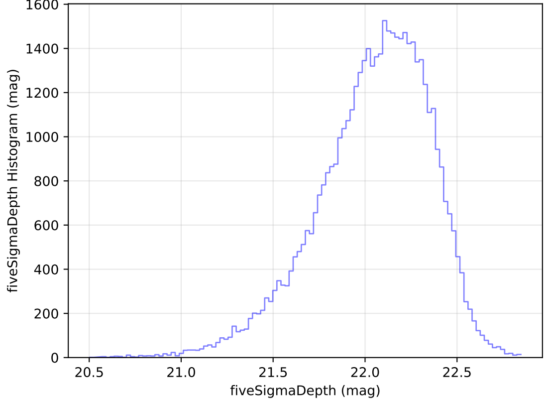
ddf_acor_sf15_lsf20_lsr20_v3.4_10yrs Yr 1 y band: fiveSigmaDepth Histogram
