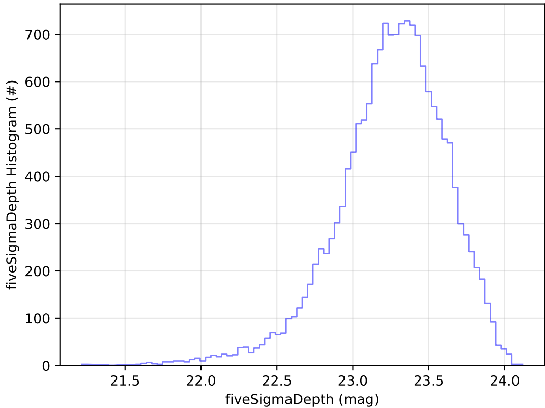
ddf_acor_sf15_lsf20_lsr20_v3.4_10yrs Yr 1 u band: fiveSigmaDepth Histogram
