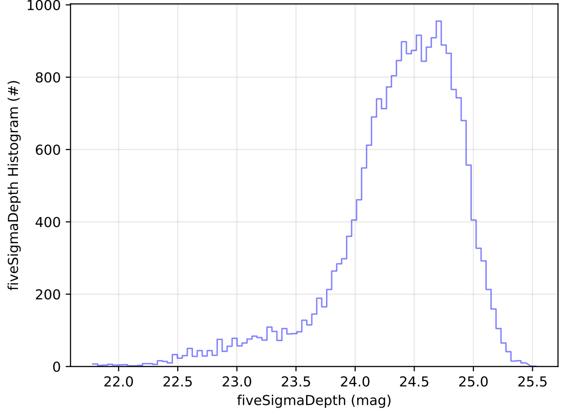
ddf_acor_sf15_lsf20_lsr20_v3.4_10yrs Yr 1 g band: fiveSigmaDepth Histogram
