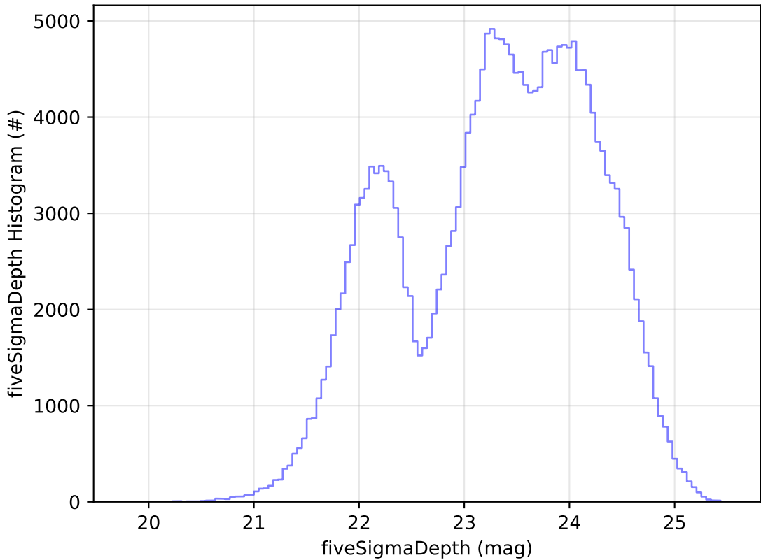
ddf_acor_sf15_lsf20_lsr20_v3.4_10yrs Yr 1 all bands: fiveSigmaDepth Histogram
