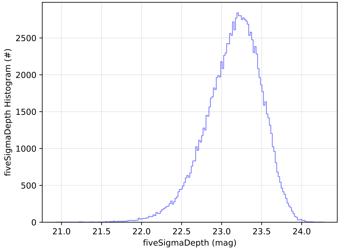
ddf_acor_sf15_lsf20_lsr20_v3.4_10yrs WFD u band: fiveSigmaDepth Histogram
