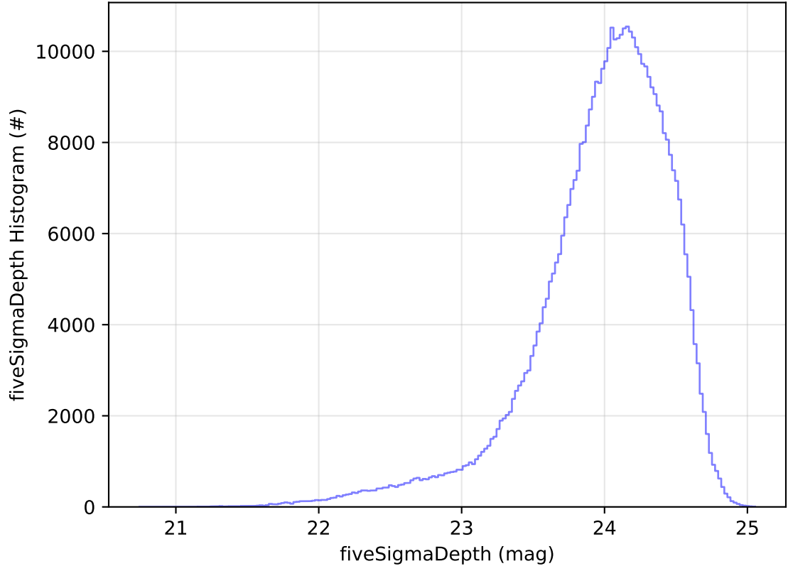
ddf_acor_sf15_lsf20_lsr20_v3.4_10yrs WFD r band: fiveSigmaDepth Histogram
