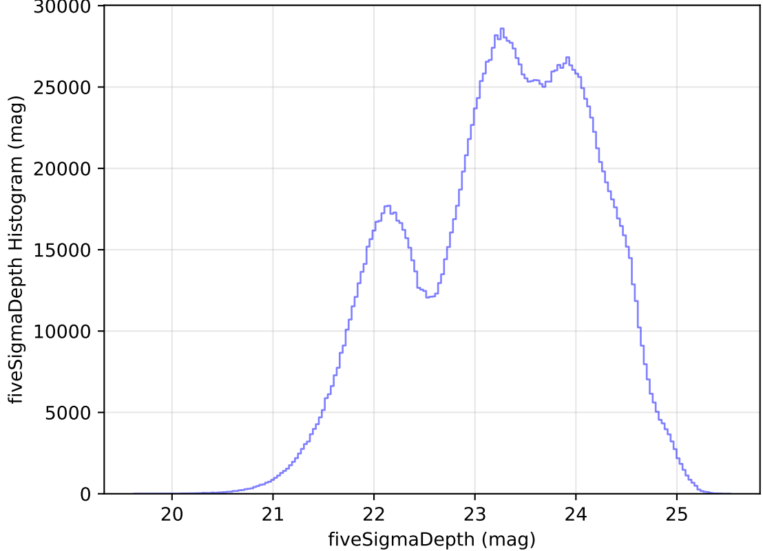
ddf_acor_sf15_lsf20_lsr20_v3.4_10yrs WFD all bands: fiveSigmaDepth Histogram
