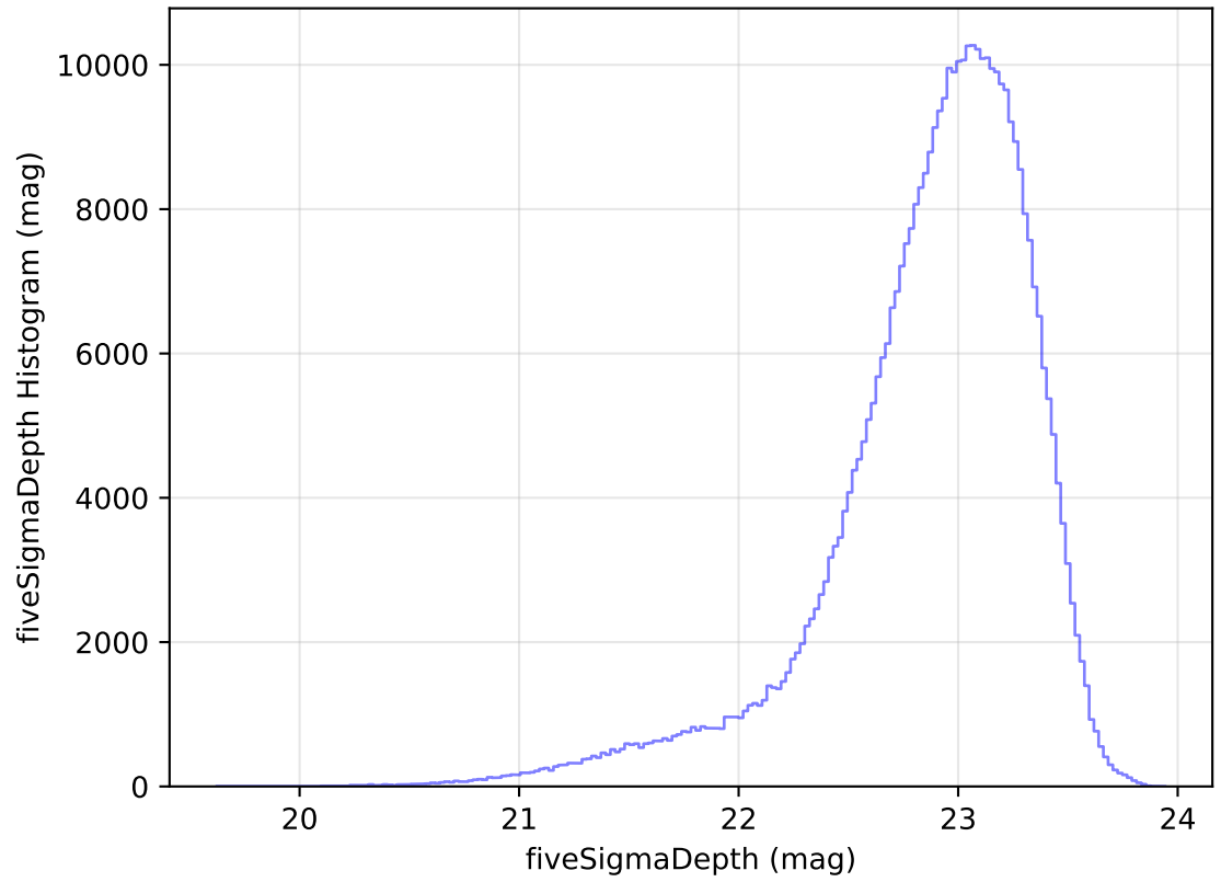
ddf_acor_sf15_lsf20_lsr20_v3.4_10yrs All sky z band: fiveSigmaDepth Histogram
