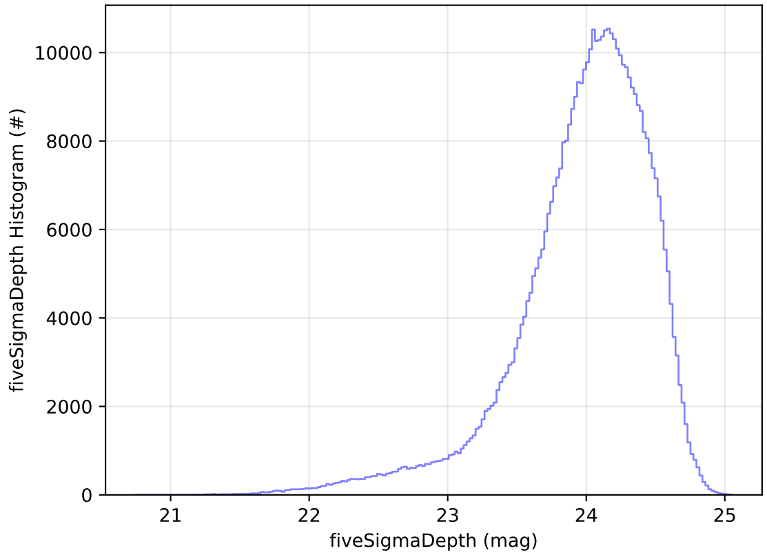
ddf_acor_sf15_lsf20_lsr20_v3.4_10yrs All sky r band: fiveSigmaDepth Histogram
