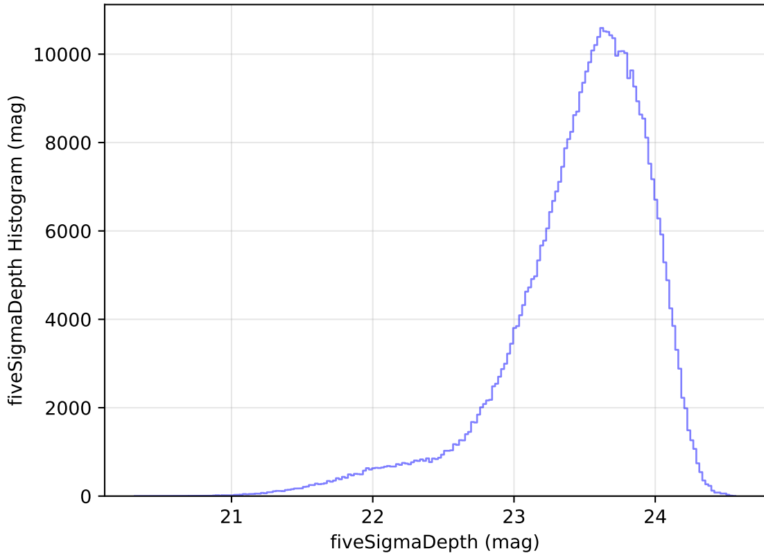
ddf_acor_sf15_lsf20_lsr20_v3.4_10yrs All sky i band: fiveSigmaDepth Histogram
