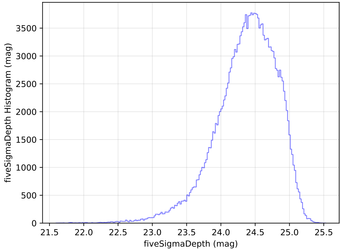
ddf_acor_sf15_lsf20_lsr20_v3.4_10yrs All sky g band: fiveSigmaDepth Histogram
