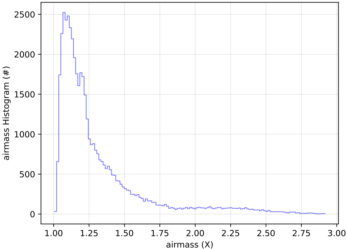
ddf_acor_sf15_lsf20_lsr20_v3.4_10yrs Yr 1 z band: airmass Histogram
