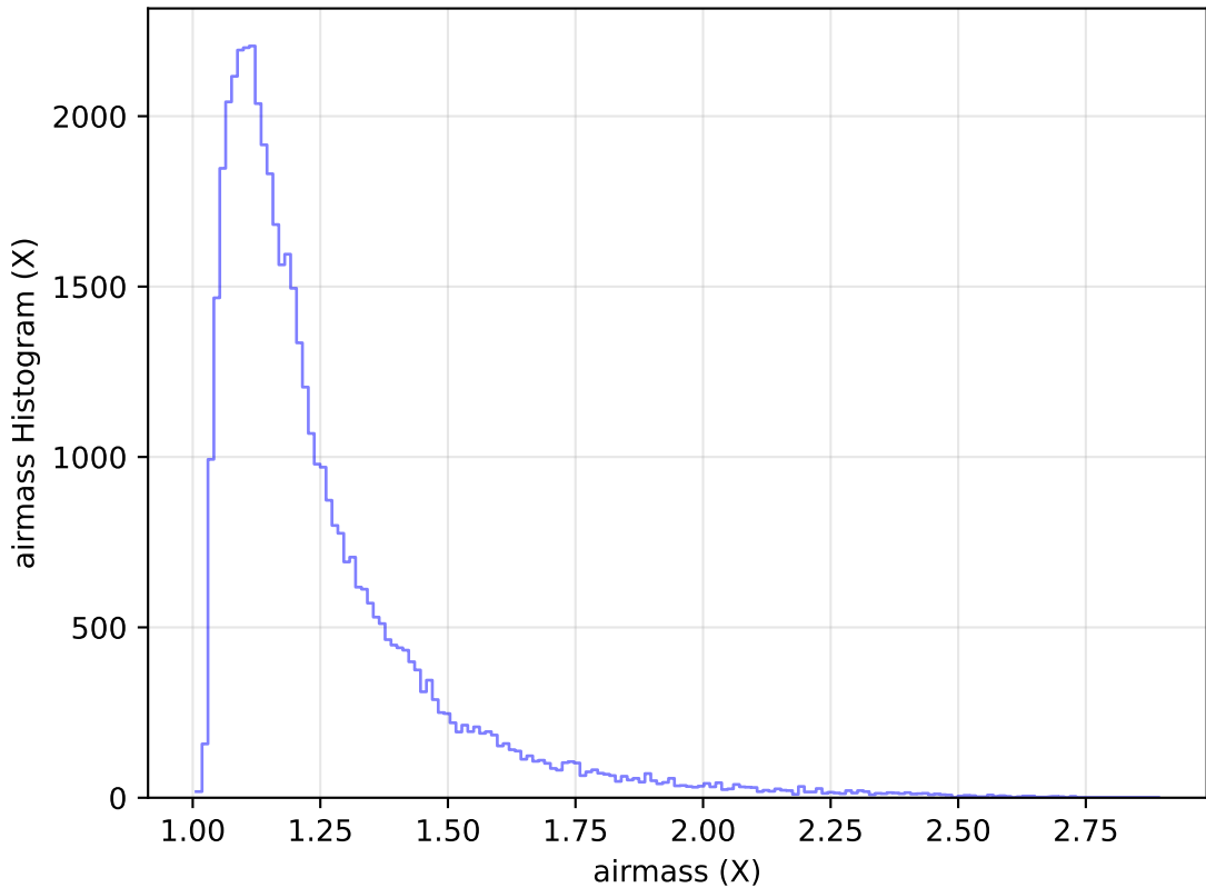
ddf_acor_sf15_lsf20_lsr20_v3.4_10yrs Yr 1 y band: airmass Histogram
