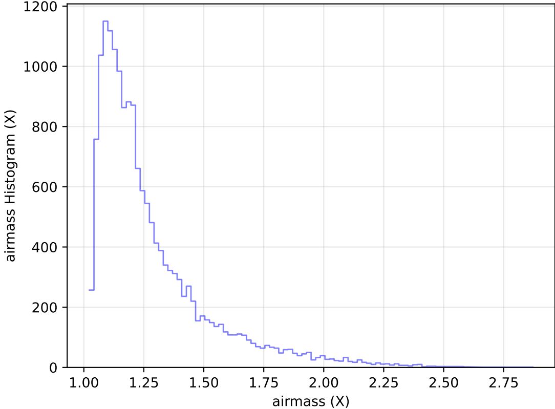
ddf_acor_sf15_lsf20_lsr20_v3.4_10yrs Yr 1 u band: airmass Histogram
