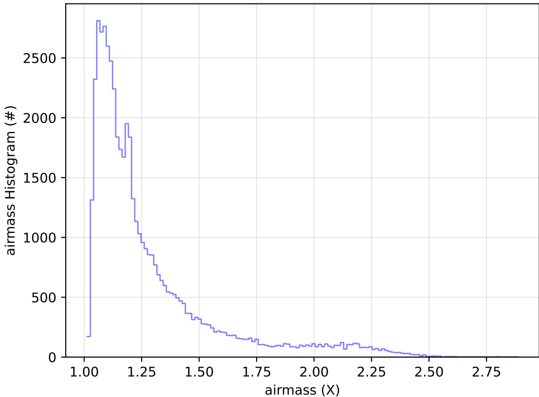
ddf_acor_sf15_ls20_lsr20_v3.4_10yrs Yr 1 r band: airmass Histogram
