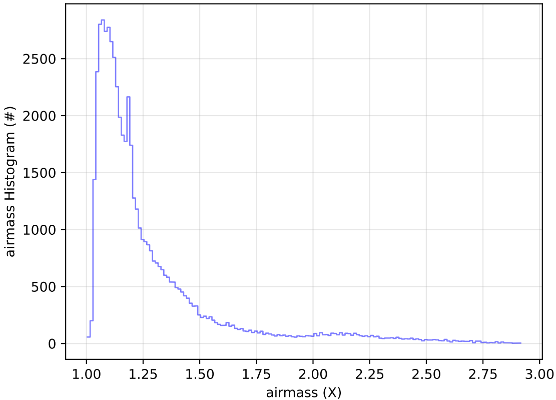
ddf_acor_sf15_lsf20_lsr20_v3.4_10yrs Yr 1 i band: airmass Histogram
