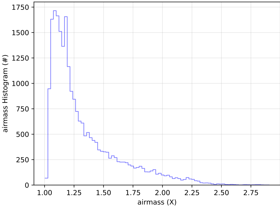
ddf_acor_sf15_lsf20_lsr20_v3.4_10yrs Yr 1 g band: airmass Histogram
