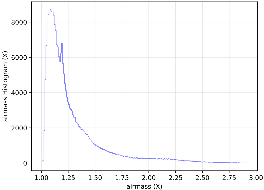
ddf_acor_sf15_lsf20_lsr20_v3.4_10yrs Yr 1 all bands: airmass Histogram
