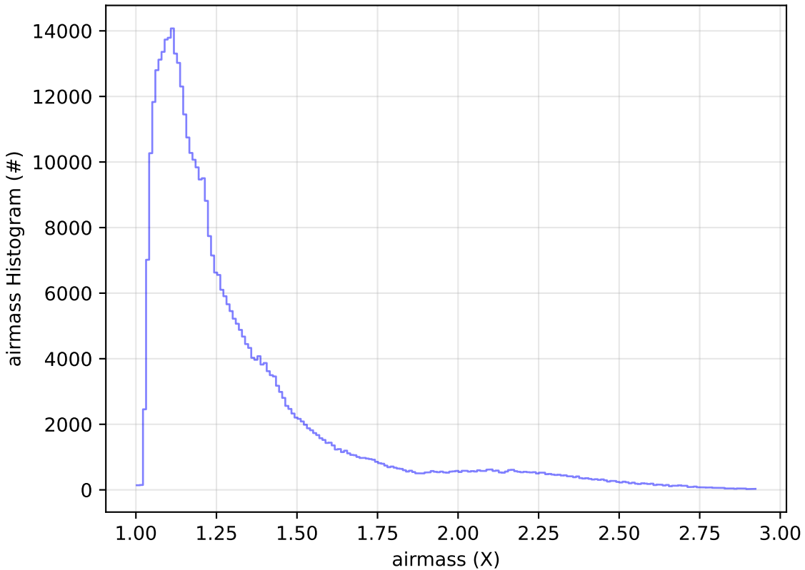
ddf_acor_sf15_lsf20_lsr20_v3.4_10yrs WFD z band: airmass Histogram
