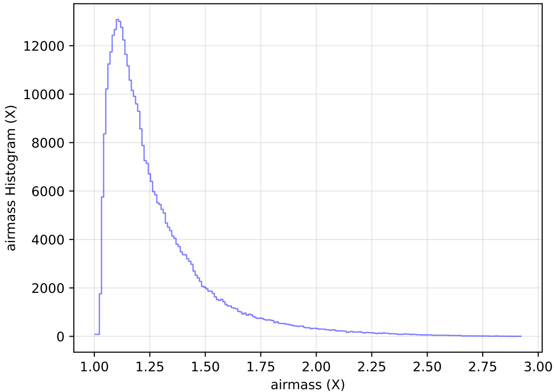
ddf_acor_sf15_lsf20_lsr20_v3.4_10yrs WFD y band: airmass Histogram
