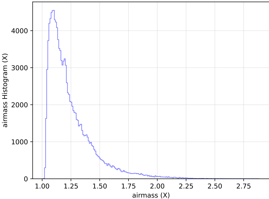
ddf_acor_sf15_lsf20_lsr20_v3.4_10yrs WFD u band: airmass Histogram
