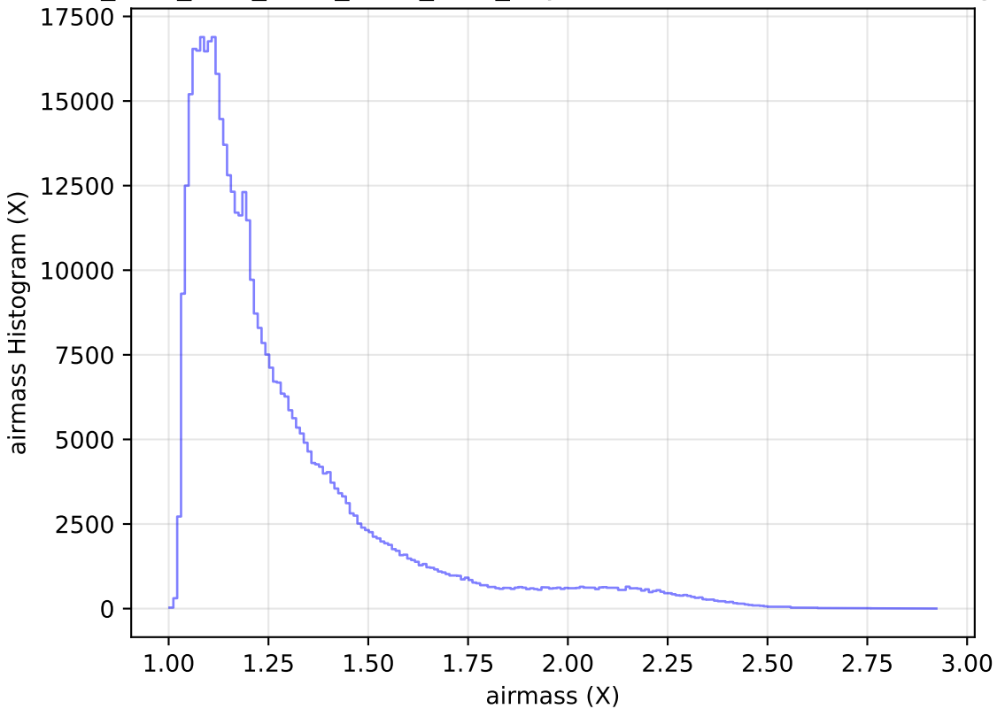
ddf_acor_sf15_lsf20_lsr20_v3.4_10yrs WFD r band: airmass Histogram
