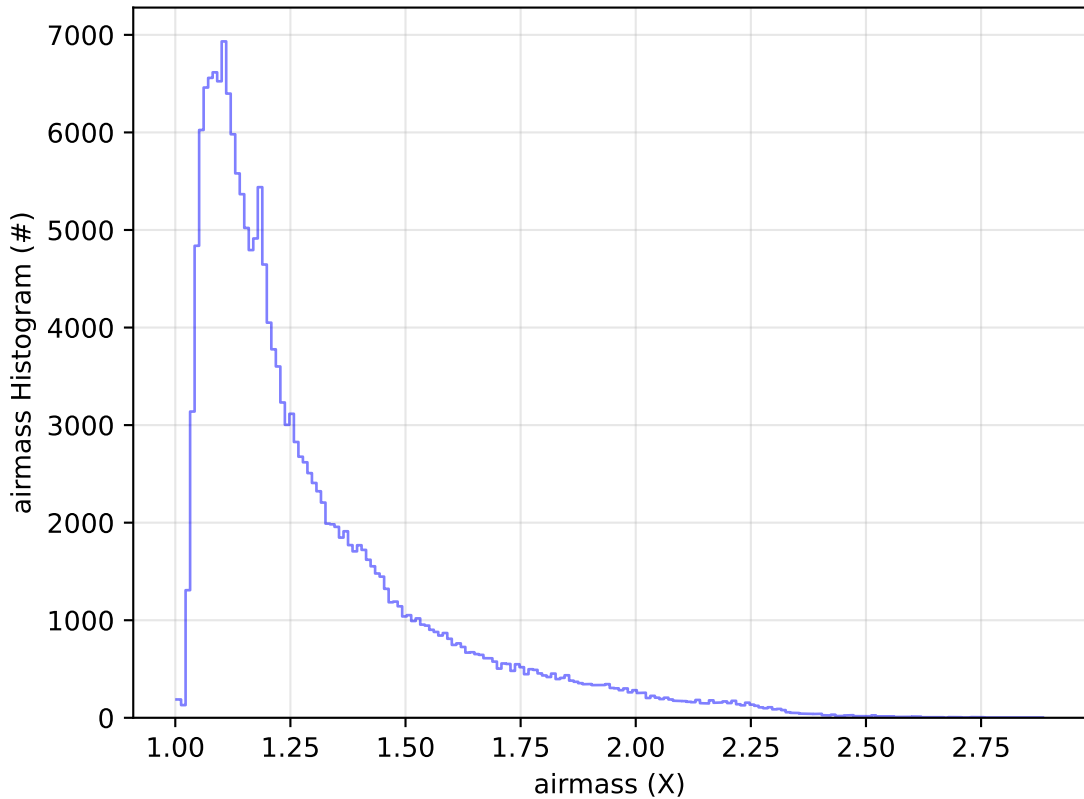
ddf_acor_sf15_lsf20_lsr20_v3.4_10yrs WFD g band: airmass Histogram
