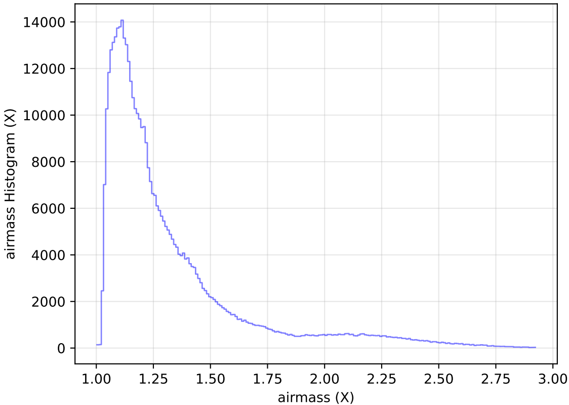
ddf_acor_sf15_lsf20_lsr20_v3.4_10yrs All sky z band: airmass Histogram
