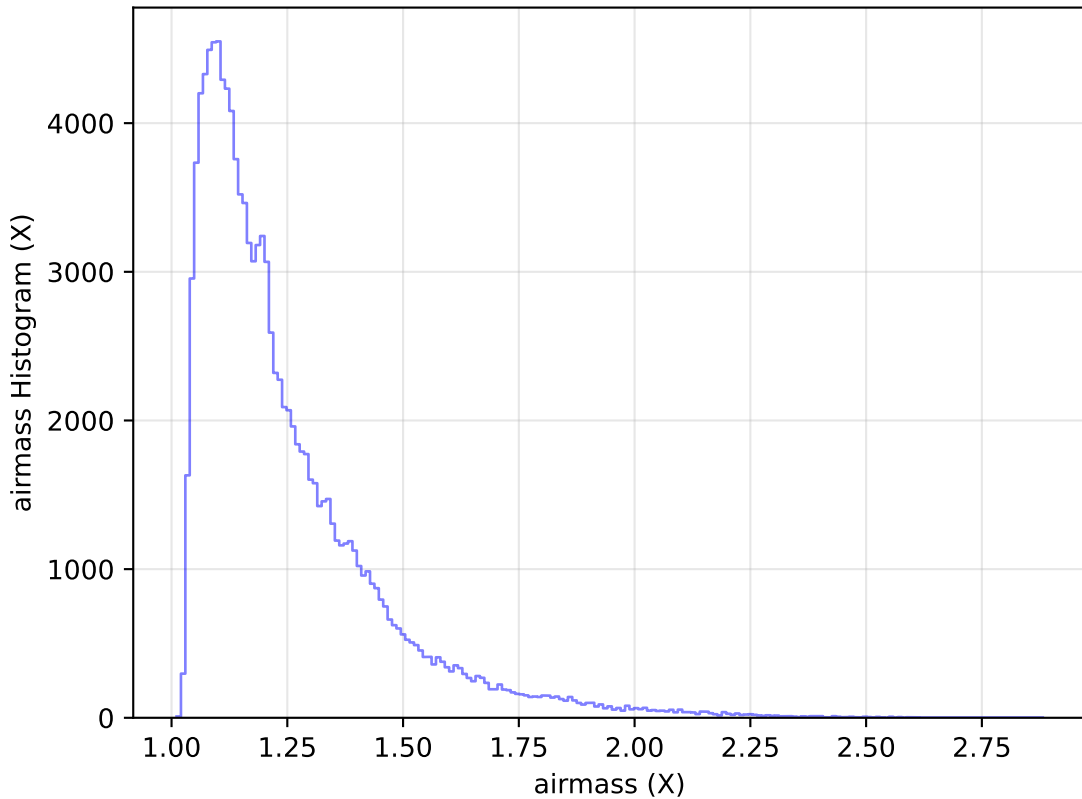
ddf_acor_sf15_lsf20_lsr20_v3.4_10yrs All sky u band: airmass Histogram
