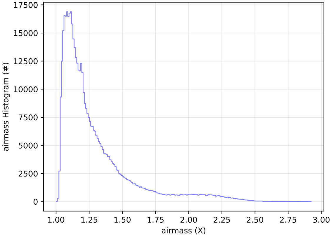
ddf_acor_sf15_lsf20_lsr20_v3.4_10yrs All sky r band: airmass Histogram
