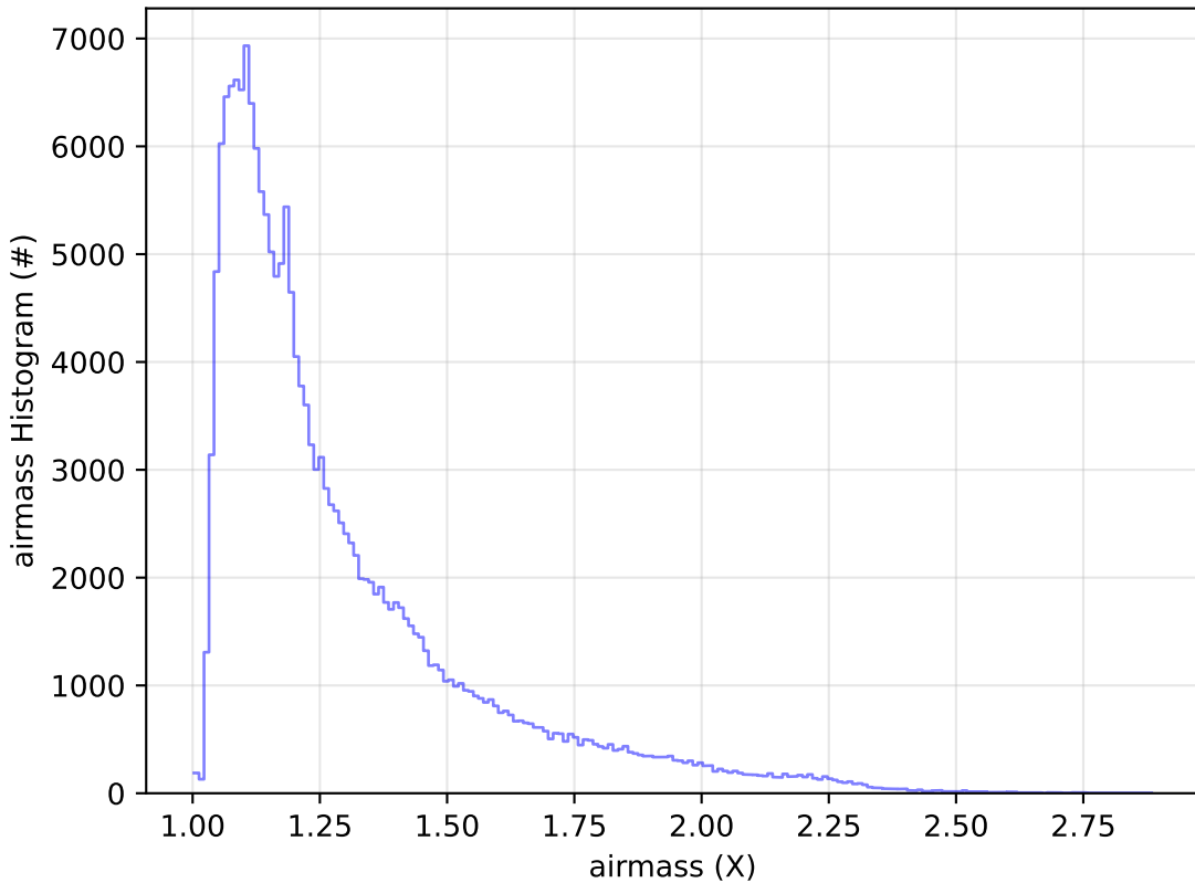
ddf_acor_sf15_lsf20_lsr20_v3.4_10yrs All sky g band: airmass Histogram
