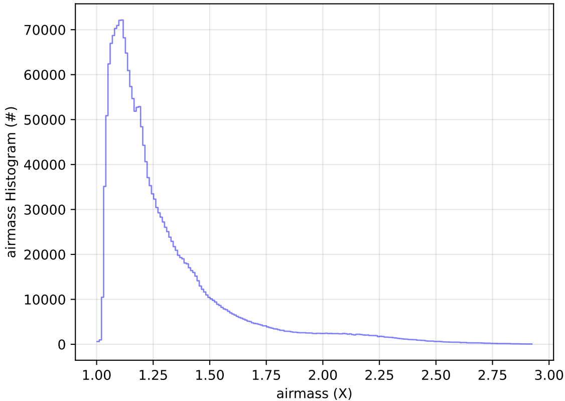
ddf_acor_sf15_lsf20_lsr20_v3.4_10yrs All sky all bands: airmass Histogram
