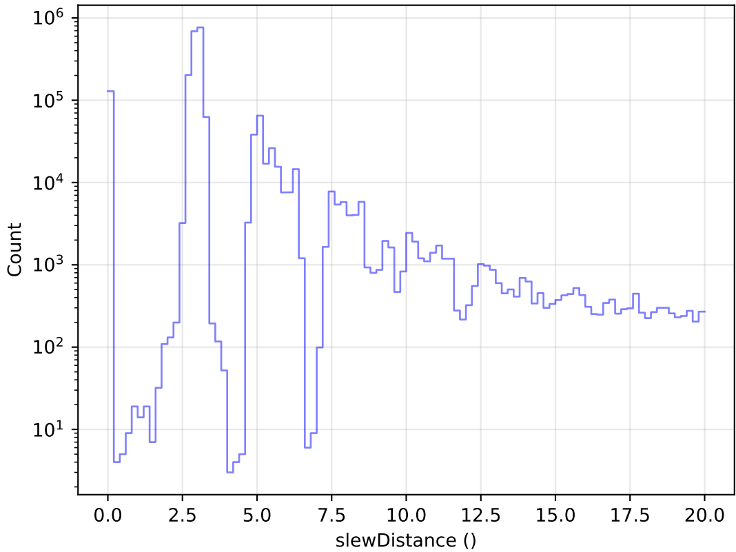
ddf_acor_sf15_lsf20_lsr20_v3.4_10yrs All visits: Zoom Slew Distance Histogram
