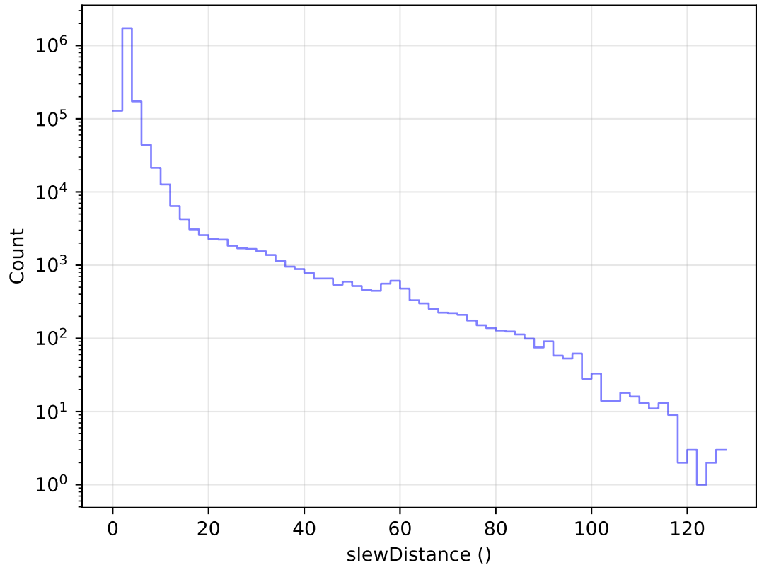
ddf_acor_sf15_lsf20_lsr20_v3.4_10yrs All visits: Slew Distance Histogram
