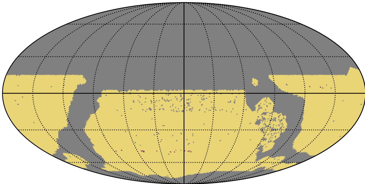
ddf_acor_sf15_lsf20_lsr20_v3.4_10yrs WFD: RapidRevisits
