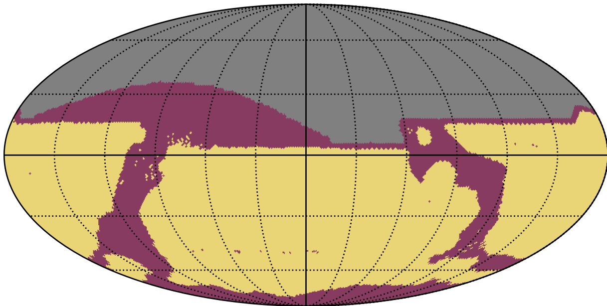
ddf_acor_sf15_lsf20_lsr20_v3.4_10yrs All sky: RapidRevisits
