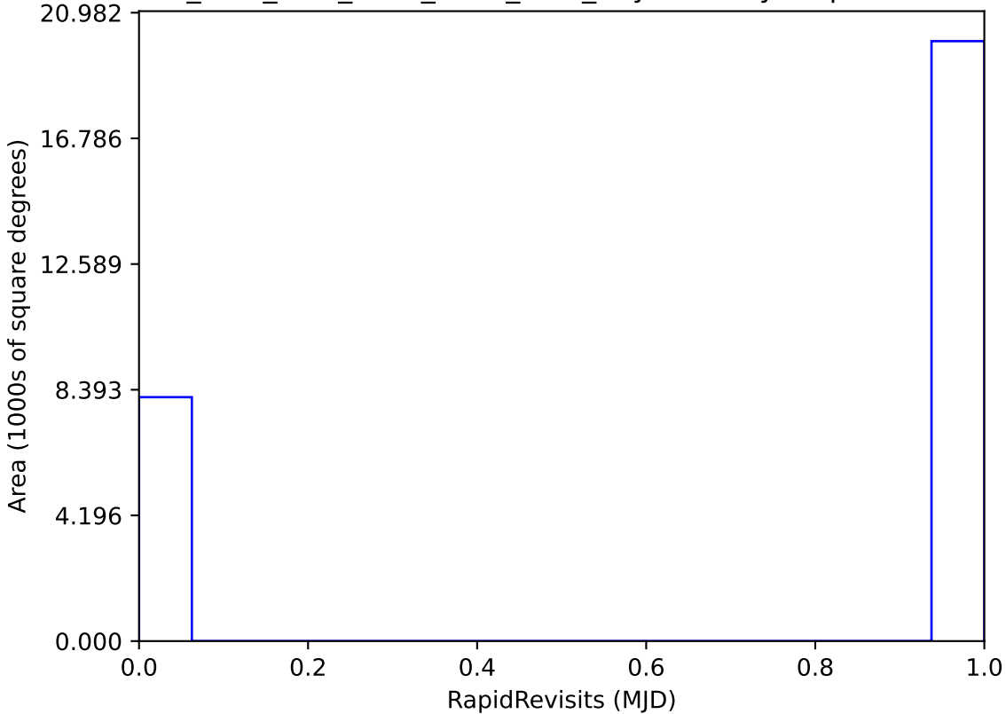
ddf_acor_sf15_lsf20_lsr20_v3.4_10yrs All sky: RapidRevisits
