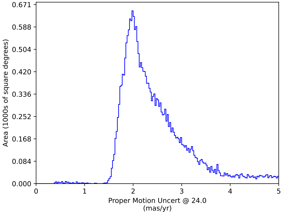
ddf_acor_sf15_lsf20_lsr20_v3.4_10yrs All sky: Proper Motion Uncert @ 24.0
