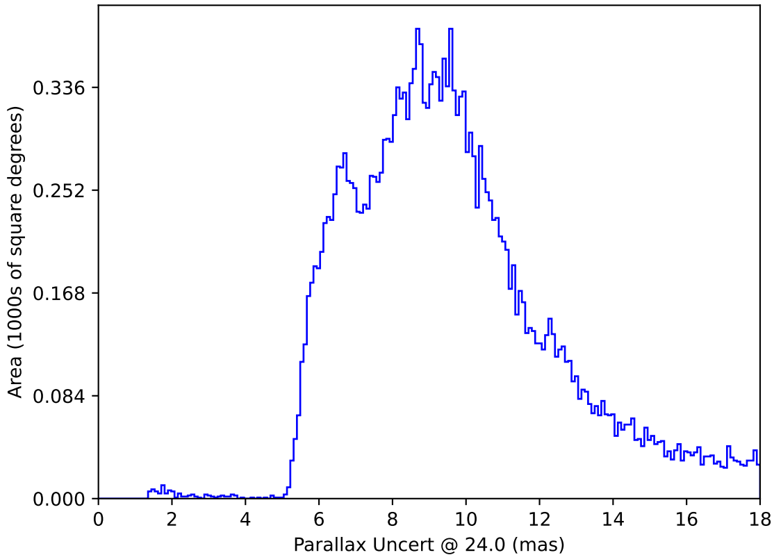
ddf_acor_sf15_lsf20_lsr20_v3.4_10yrs All sky: Parallax Uncert @ 24.0
