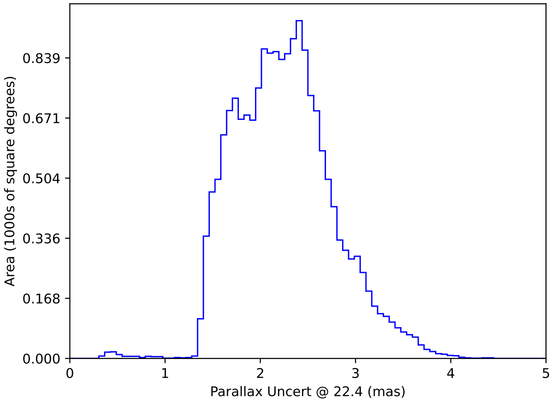
ddf_acor_sf15_lsf20_lsr20_v3.4_10yrs WFD: Parallax Uncert @ 22.4
