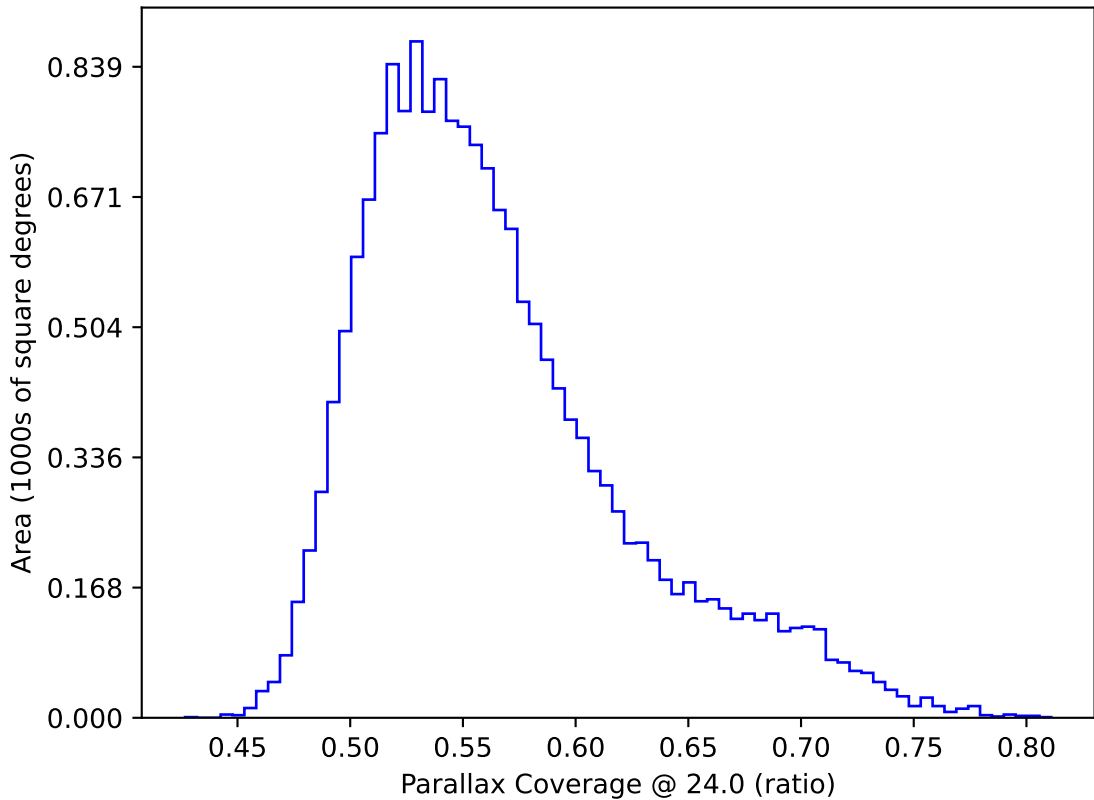
ddf_acor_sf15_lsf20_lsr20_v3.4_10yrs WFD: Parallax Coverage @ 24.0
