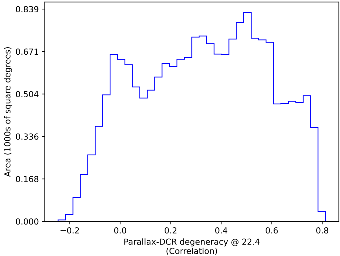
ddf_acor_sf15_lsf20_lsr20_v3.4_10yrs WFD: Parallax-DCR degeneracy @ 22.4
