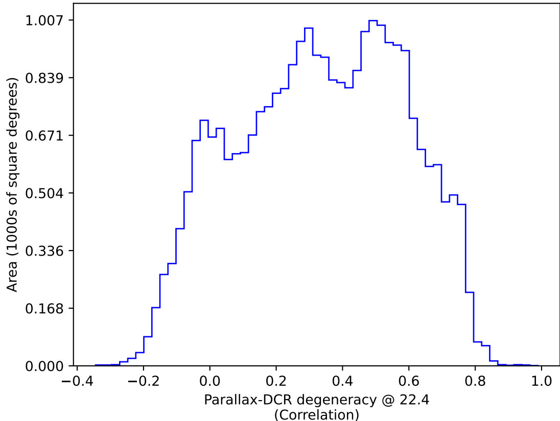
ddf_acor_sf15_lsf20_lsr20_v3.4_10yrs All sky: Parallax-DCR degeneracy @ 22.4
