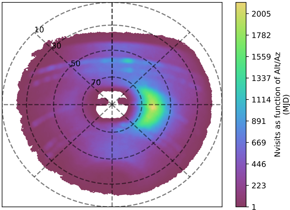
ddf_acor_sf15_lsf20_lsr20_v3.4_10yrs y band: Nvisits as function of Alt/Az
