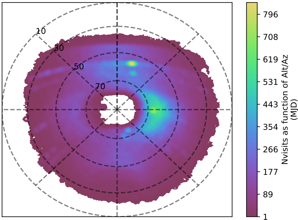
ddf_acor_sf15_lsf20_lsr20_v3.4_10yrs u band: Nvisits as function of Alt/Az
