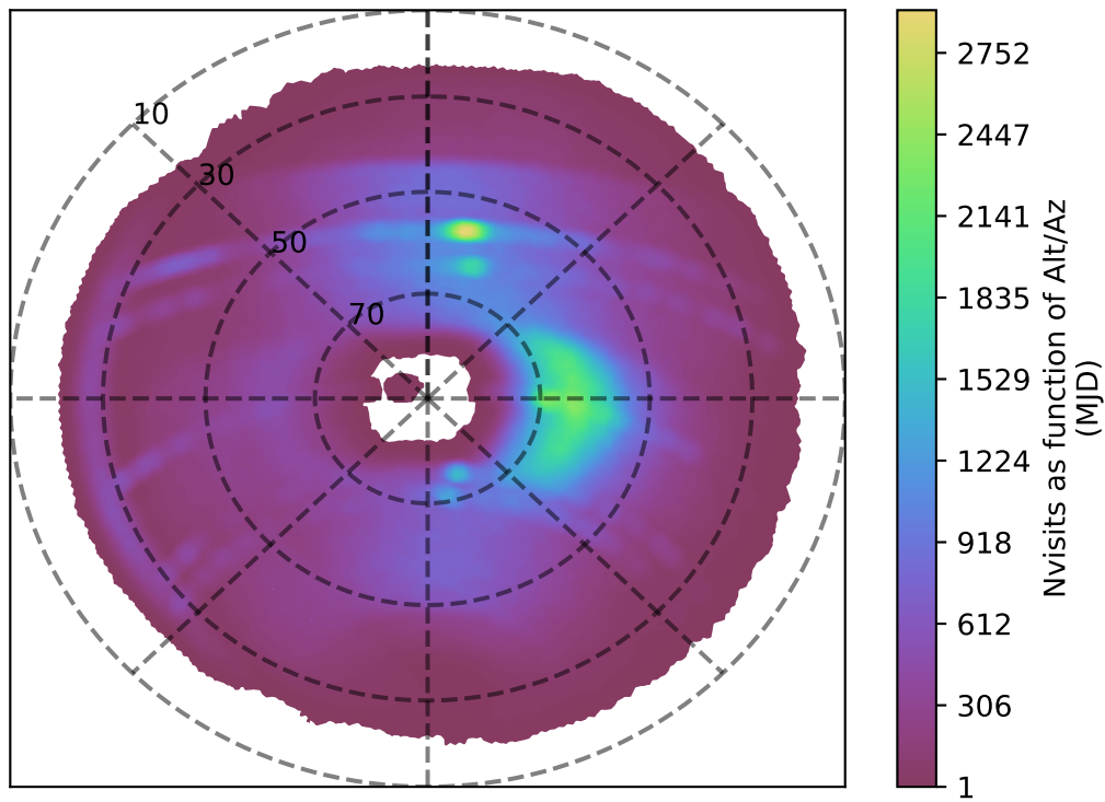
ddf_acor_sf15_lsf20_lsr20_v3.4_10yrs r band: Nvisits as function of Alt/Az
