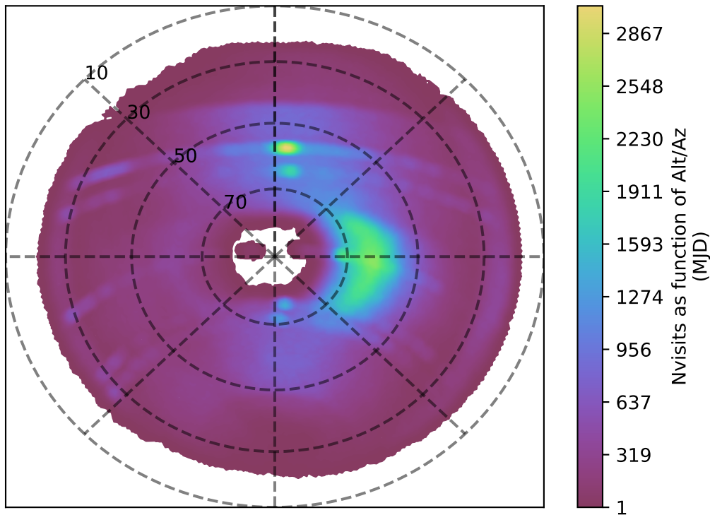
ddf_acor_sf15_lsf20_lsr20_v3.4_10yrs i band: Nvisits as function of Alt/Az
