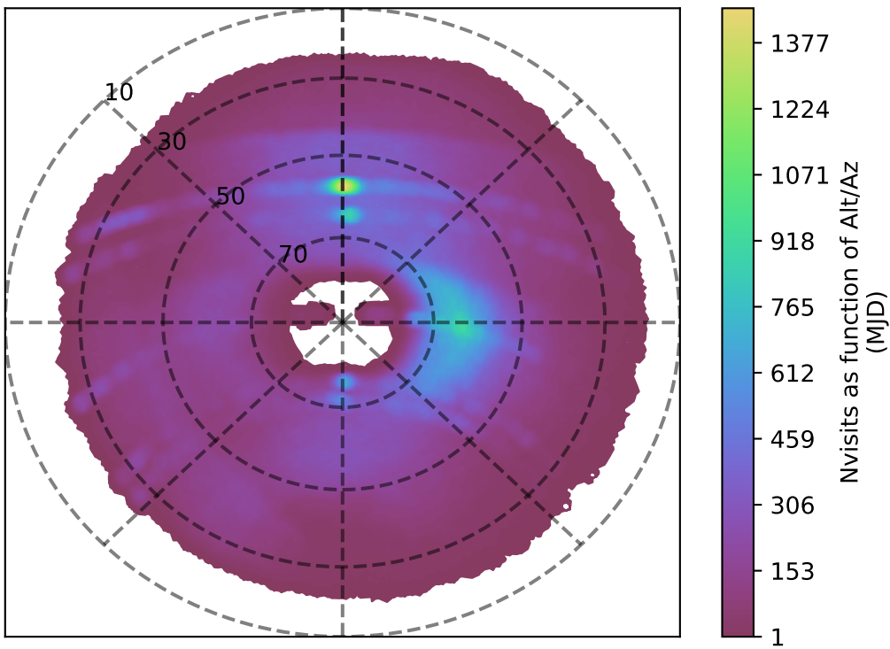
ddf_acor_sf15_lsf20_lsr20_v3.4_10yrs g band: Nvisits as function of Alt/Az
