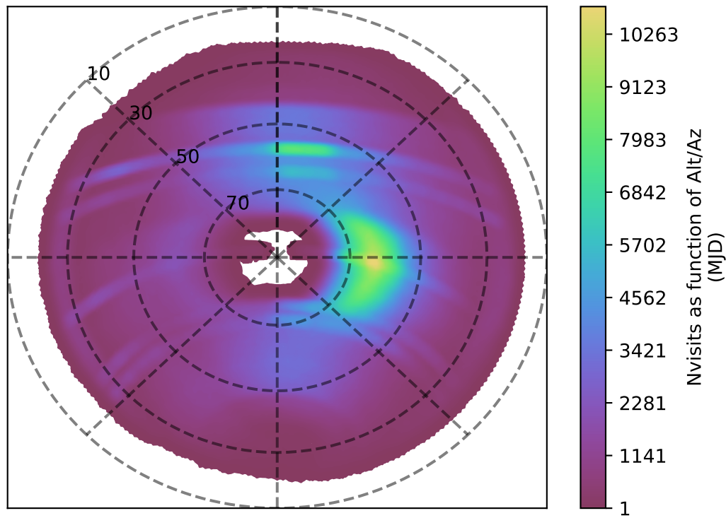
ddf_acor_sf15_lsf20_lsr20_v3.4_10yrs all bands: Nvisits as function of Alt/Az
