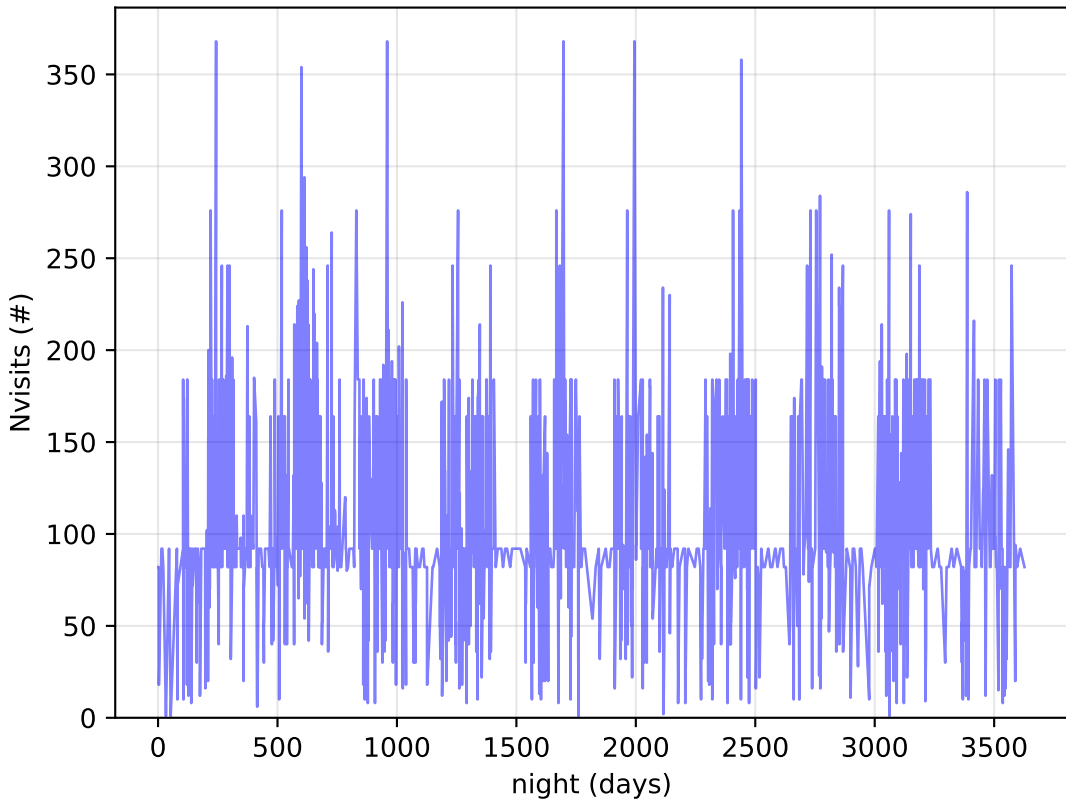
ddf_acor_sf15_lsf20_lsr20_v3.4_10yrs DDF: Nvisits
