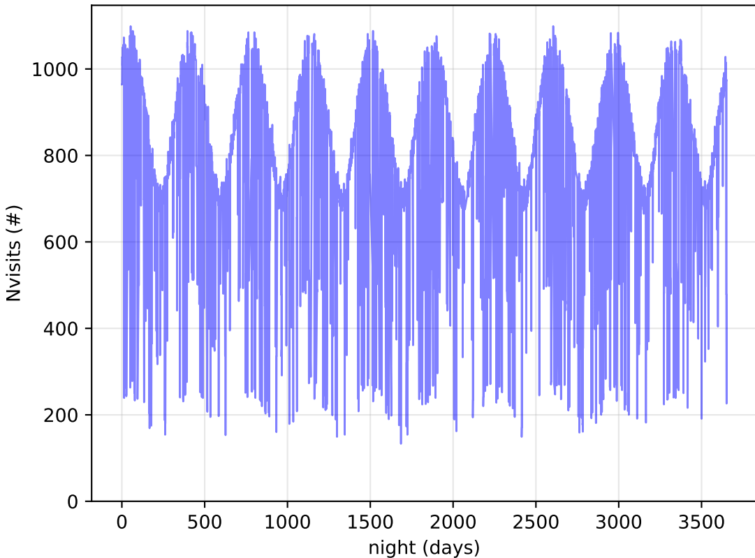
ddf_acor_sf15_ls20_lsr20_v3.4_10yrs All visits: Nvisits
