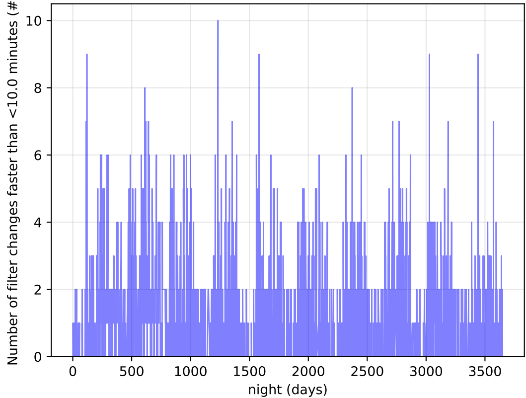
ddf_acor_sf15_Isf20_Isr20_v3.4_10yrs Per Night: Number of filter changes faster than <10.0 minutes
